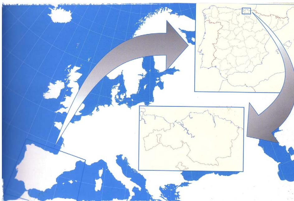
Fig. 1. The study area, Bizkaia, north of Spain.
